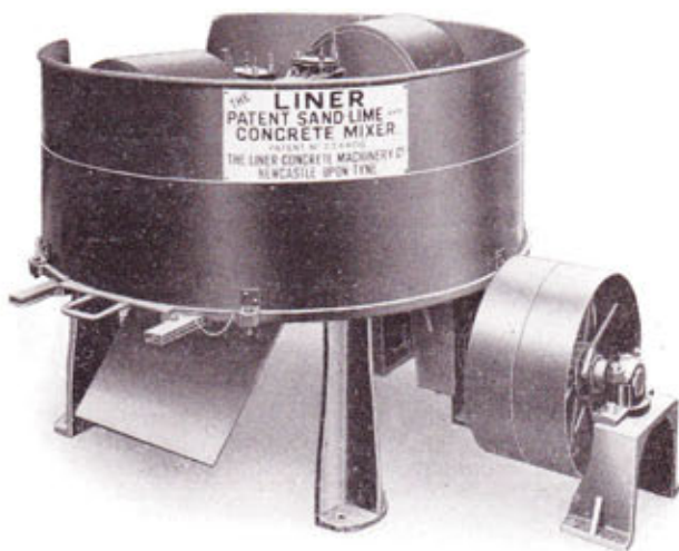
No. 2 size, with 5' 6" diameter Pan, fixed model, requiring 7 H.P. to drive. Total weight, 35 cwt. A 60 bricklayer unit, with two operators.
