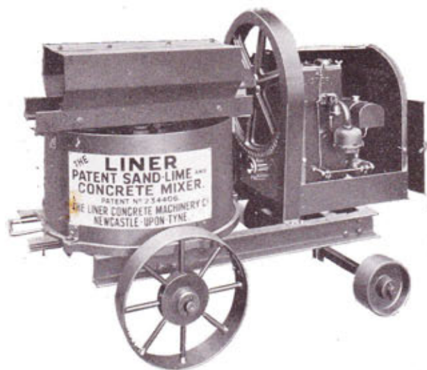
No. 0 Size, with 2' 6" diameter Pan, direct-driven by 1½ H.P. "Lister" Petrol Engine in Steel Housing, with lift-off sides—one side removed. Total weight 15 cwt. Keeps 12 to 15 bricklayers supplied with sand-lime mortar.
