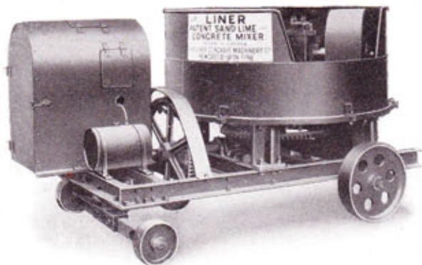
No. 1 size, with 4' 6" diameter Pan, direct-driven by 3 H.P. "Lister" Petrol Engine, in Steel Housing, with lift-off sides. Total weight, 30 cwt. A thirty bricklayer unit, with one operator.
